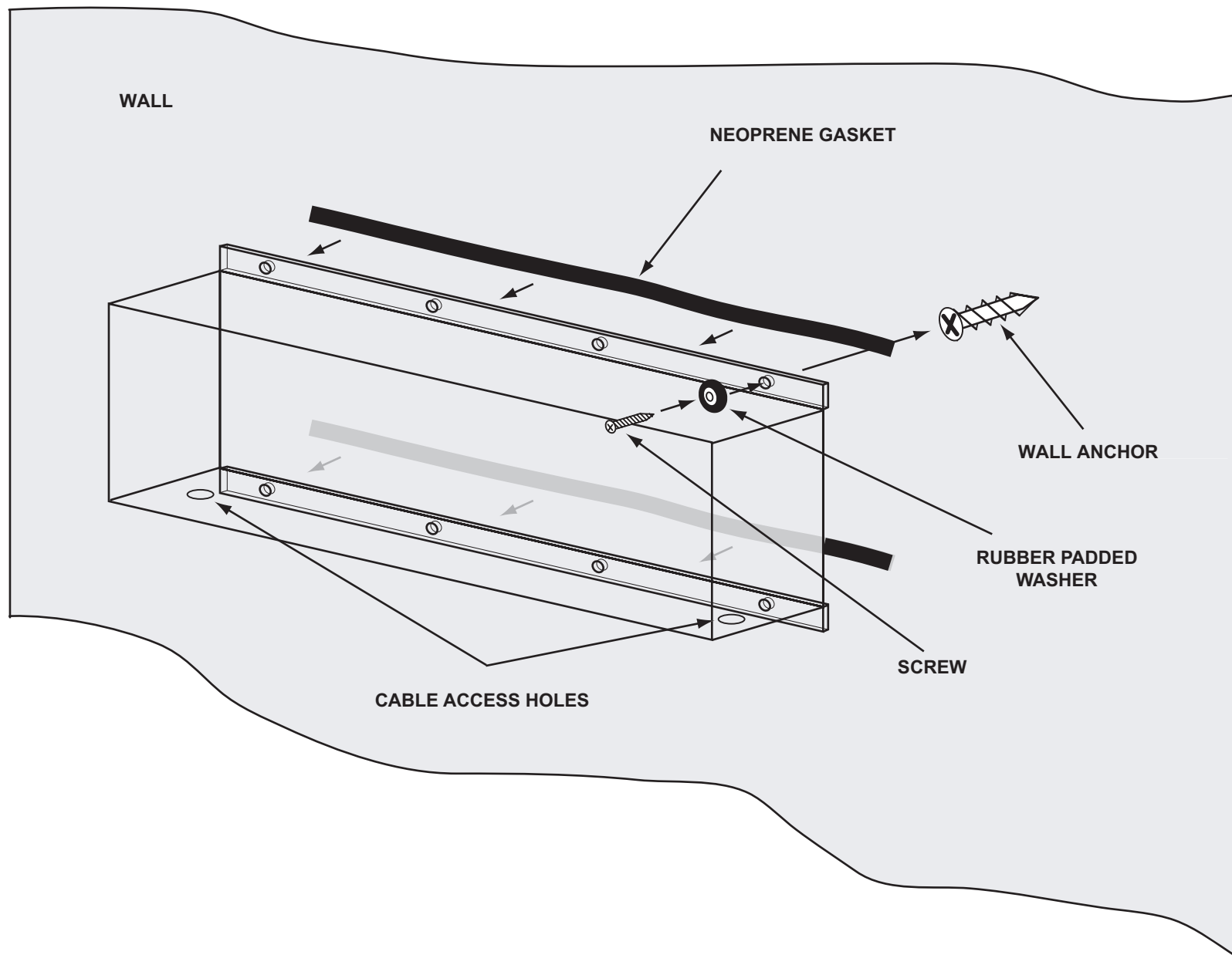
ACRYLIC AND LEXAN GUARD / COVER INSTALLATION
