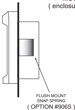
OPTIONAL FLUSH MOUNT METHOD ( enclosure option # 732FL )
