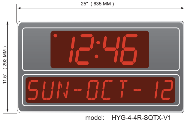
model: HYG-4-4R-SQTX-V1
