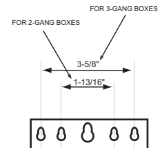
KEYHOLE SET VIEW IN TYPICAL BACK PANEL
