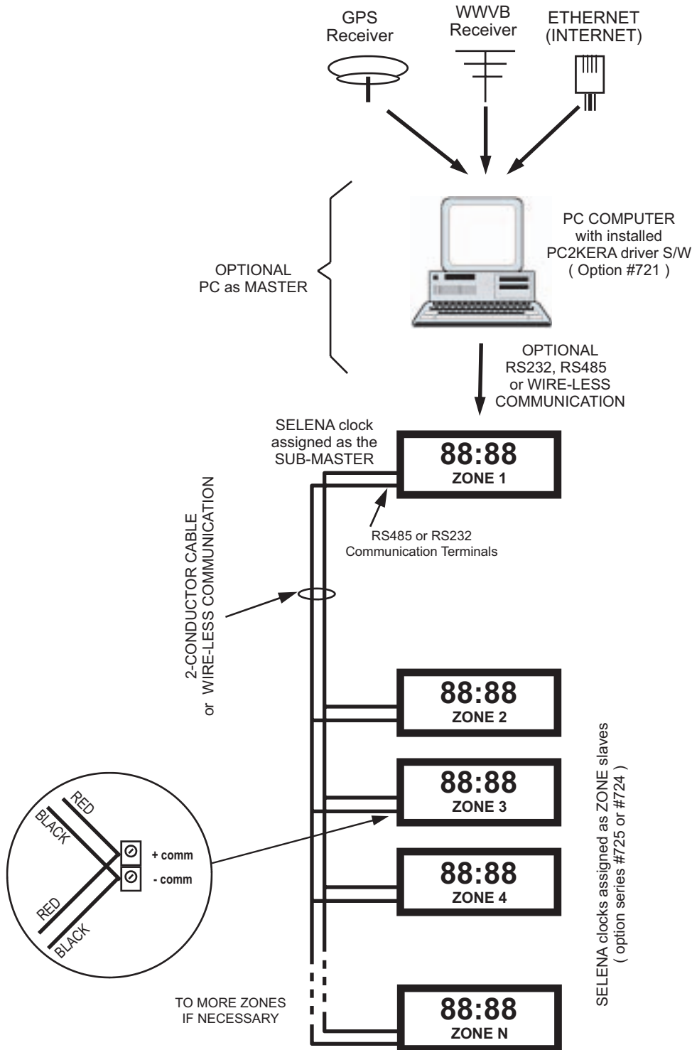
EXAMPLE OF MULTI-ZONE SYSTEM WITH ZONE CLOCKS HOUSED IN SEPARATE ENCLOSURES
