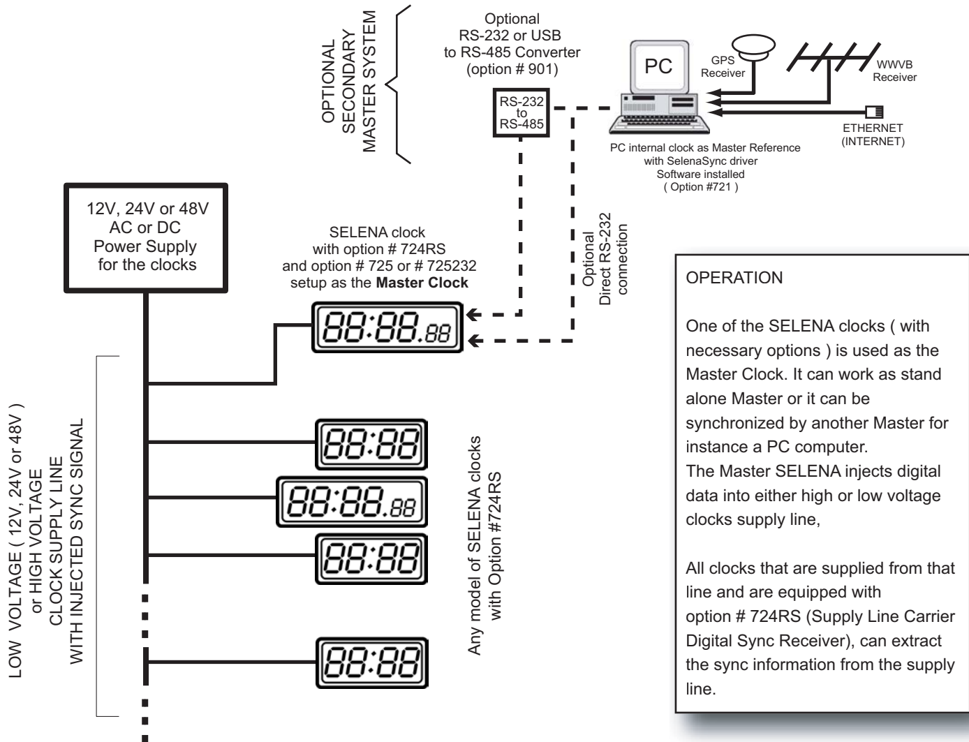
Configuration with Supply Line Carrier Digital Communication and SELENA as the Master Clock with optional PC as the Master Reference
