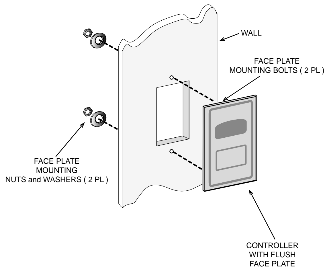
FLUSH MOUNTING IN WALL
