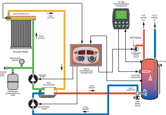
SPLIT PRESSURIZED SYSTEM USING EXTERNAL HEAT EXCHANGER AND ONE STANDARD TANK
