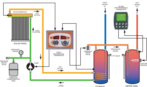
SPLIT PRESSURIZED SYSTEM USING ONE STORAGE TANK WITH INTERNAL HEAT EXCHANGER AND A SERVICE TANK WITH ELECTRIC BOOSTER
