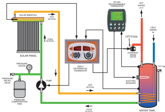
SPLIT PRESSURIZED SYSTEM USING ONE TANK WITH INTERNAL HEAT EXCHANGER
