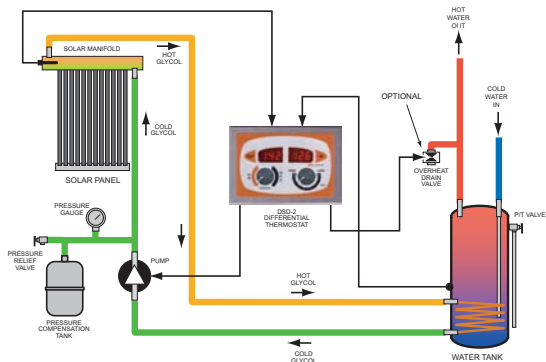
SIMPLE SPLIT PRESSURIZED SYSTEM USING ONE TANK WITH INTERNAL HEAT EXCHANGER
