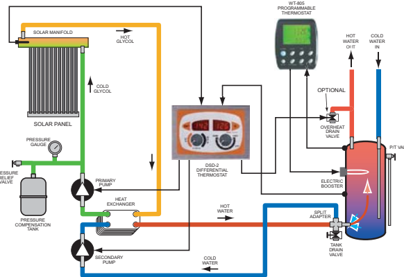
SPLIT PRESSURIZED SYSTEM USING EXTERNAL HEAT EXCHANGER AND ONE STANDARD TANK
