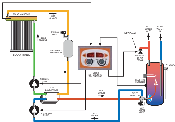
SIMPLE SPLIT DRAINBACK SYSTEM USING EXTERNAL HEAT EXCHANGER AND ONE STANDARD TANK
