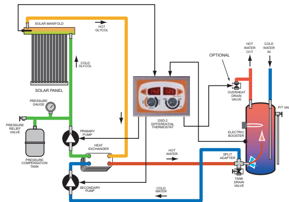
SIMPLE SPLIT PRESSURIZED SYSTEM USING EXTERNAL HEAT EXCHANGER AND ONE STANDARD TANK
