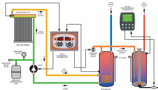
SPLIT PRESSURIZED SYSTEM USING ONE STORAGE TANK WITH INTERNAL HEAT EXCHANGER AND A SERVICE TANK WITH GAS BOOSTER
