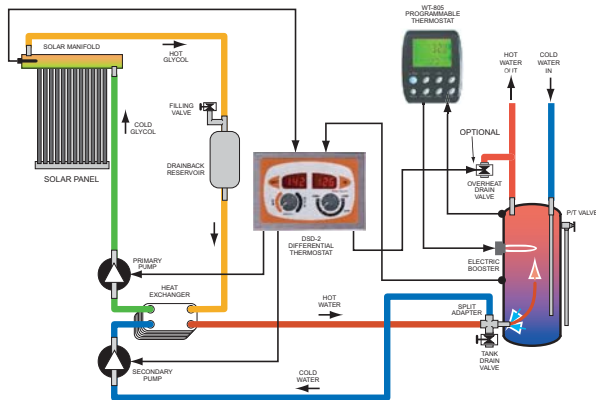
SPLIT DRAINBACK SYSTEM USING EXTERNAL HEAT EXCHANGER AND ONE STANDARD TANK
